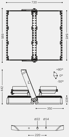
AP10-L Asymmetric Extra Forward - Left
